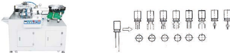
SF-508A Forming foot cutting machine
