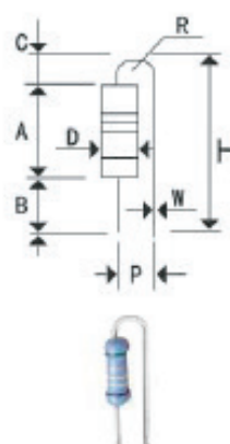
Vertical molding-F type
